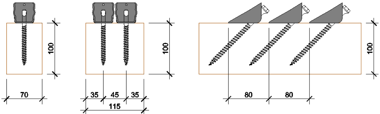
Figure 1.1.j Minimum distances and dispositions for LATERLITE CONNETTORE CENTROSTORICO LEGNO connector with screw 10x160 and wood with density < 420 kg/m 3
