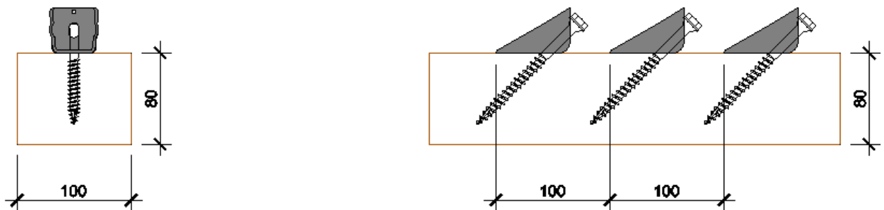
Figure 1.1.m Minimum distances and dispositions for LATERLITE CONNETTORE CENTROSTORICO LEGNO connector with screw 10x133 and wood with density < 500 kg/m 3
