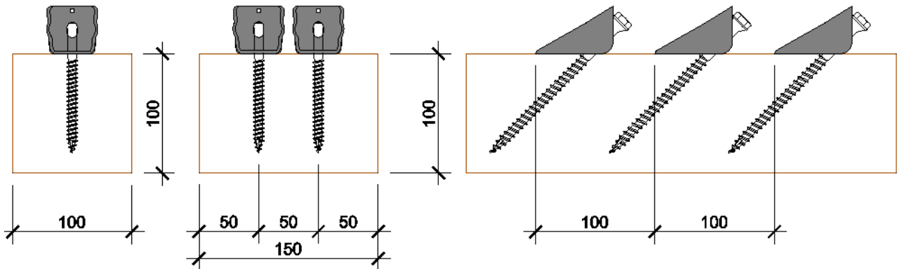
Figure 1.1.k Minimum distances and dispositions for LATERLITE CONNETTORE CENTROSTORICO LEGNO connector with screw 10x160 and wood with density < 500 kg/m 3
