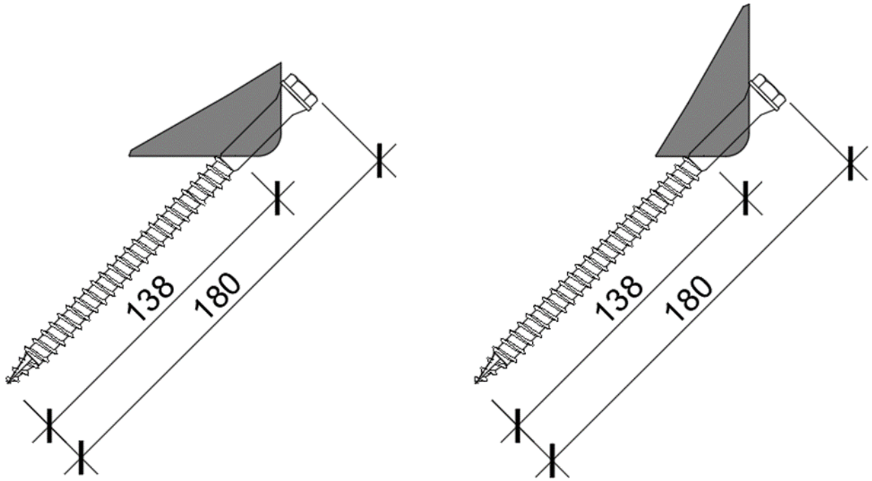
Figure 1.1.h LATERLITE CONNETTORE CENTROSTORICO LEGNO with 12x180 screw in two possibly configurations
