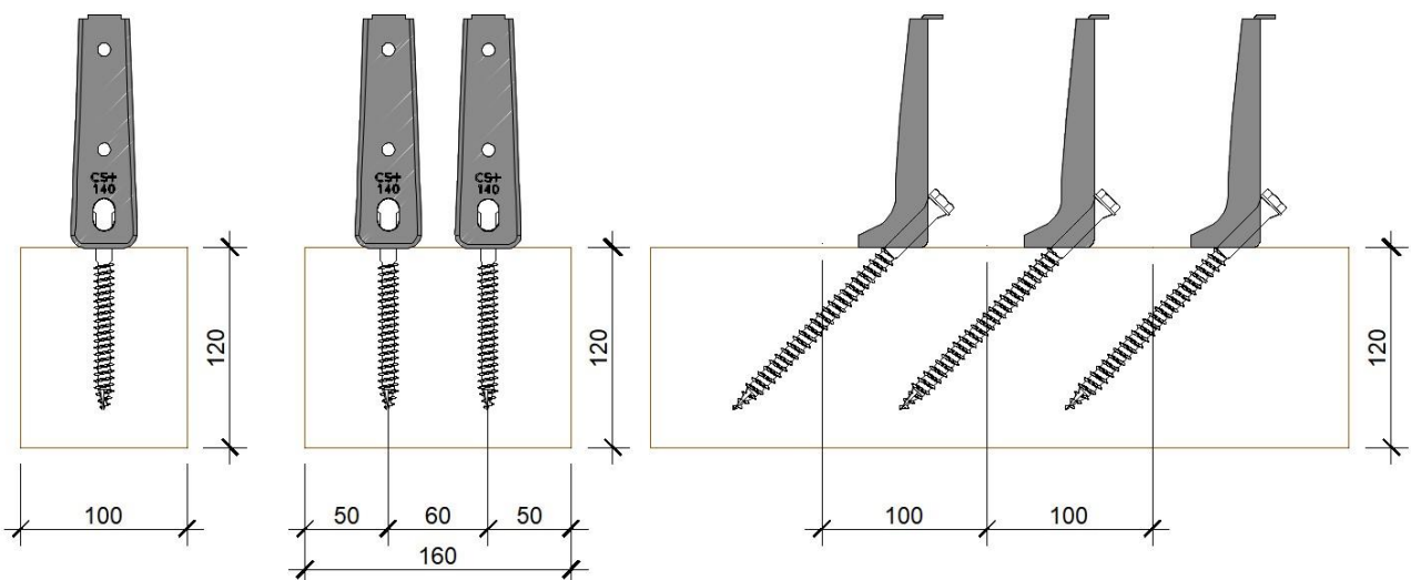
Figure 1.1.p Minimum distances and dispositions for LATERLITE CONNETTORE CENTROSTORICO LEGNO H140 connector with screw 12x180
