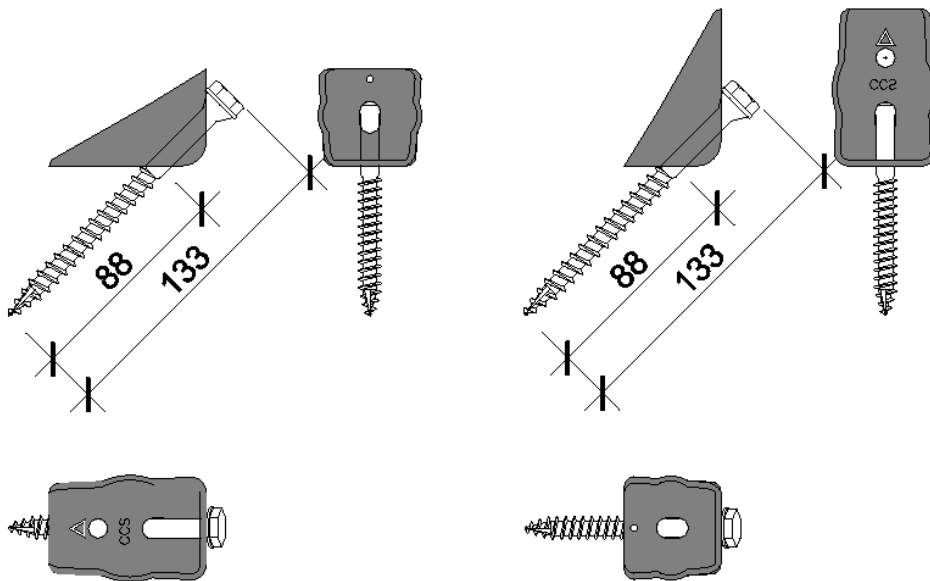
Figure 1.1.g LATERLITE CONNETTORE CENTROSTORICO LEGNO with 10x133 screw in two possibly configurations
