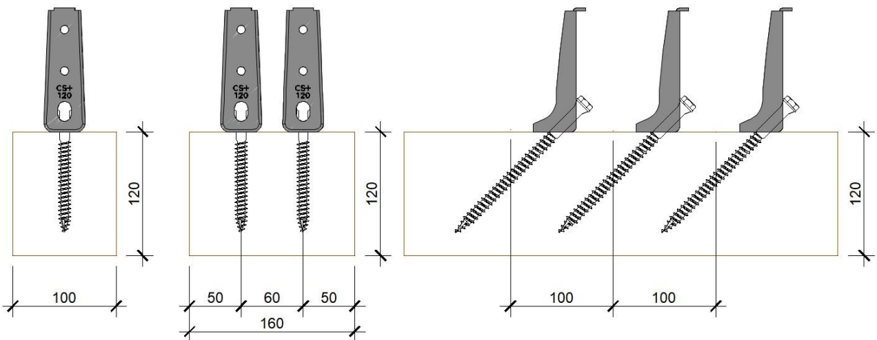
Figure 1.1.o Minimum distances and dispositions for LATERLITE CONNETTORE CENTROSTORICO LEGNO H120 connector with screw 12x180
