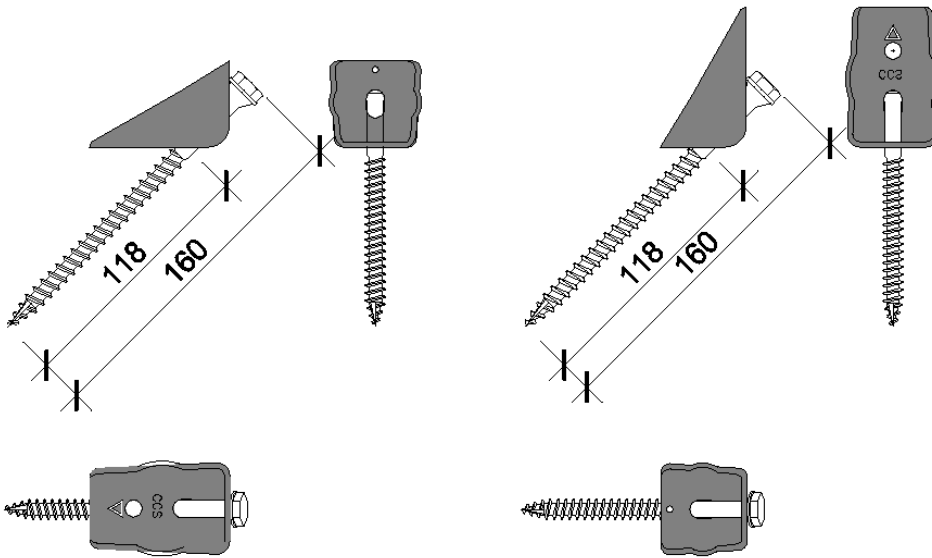
Figure 1.1.f LATERLITE CONNETTORE CENTROSTORICO LEGNO with 10x160 screw in two possibly configurations
