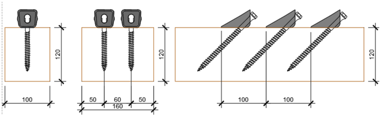
Figure 1.1.n Minimum distances and dispositions for LATERLITE CONNETTORE CENTROSTORICO LEGNO connector with screw 12x180
